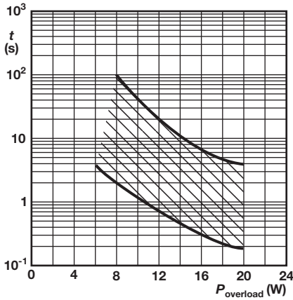
NFR25H This graph is based on measured data which may deviate according to the application. Fusing Characteristics: \leq 1 \Omega
