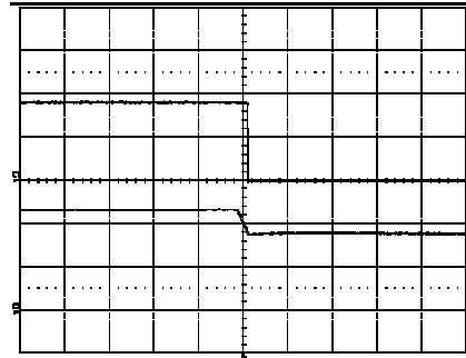
Shut-down enabled by disconnecting V_I at: T_{ref} = +25^\circ\text{C} , I_O = 6\text{ A} resistive load, V_I = 12.0\text{ V} . Top trace: output voltage (1.0 V/div.). Bottom trace: input voltage (5 V/div.). Time scale: 10.0 ms/div.
