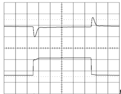
Output voltage response to load current step- change (3-6-3 A) at: T_{ref} = +25^\circ\text{C} , V_I = 12.0\text{ V} . Top trace: output voltage (100mV/div.). Bottom trace: load current (2 A/div.). Time scale: 0.1 ms/div.
