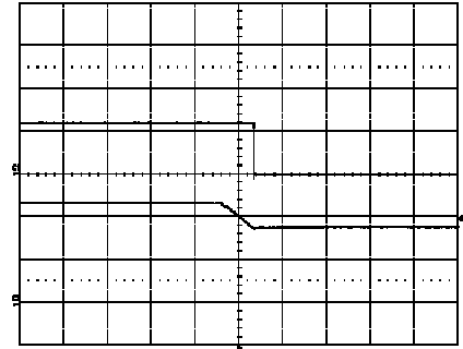
Shut-down enabled by disconnecting V_i at: T_{ref} = +25^{\circ}\text{C} , I_O = 6\text{ A} resistive load, V_i = 12.0\text{ V} . Top trace: output voltage (1.0 V/div.). Bottom trace: input voltage (5 V/div.). Time scale: 5.0 ms/div.
