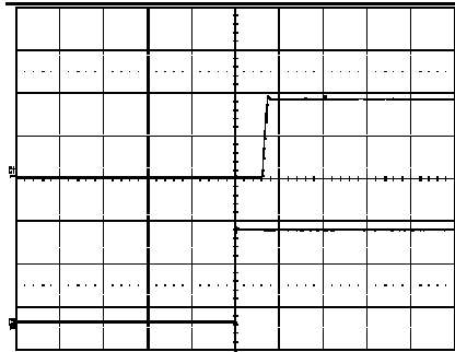
Start-up enabled by connecting V_I at: T_{ref} = +25^\circ\text{C} , I_O = 6\text{ A} resistive load, V_I = 12.0\text{ V} . Top trace: output voltage (1.0 V/div.). Bottom trace: input voltage (5 V/div.). Time scale: 20 ms/div.
