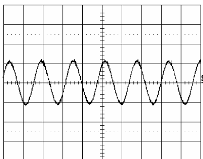
Output voltage ripple (20mV/div.) at: T_{ref} = +25^\circ\text{C} , I_O = 6\text{ A} resistive load, V_I = 12.0\text{ V} . Time scale: 2 \mu\text{s} /div. See the filter in the Output ripple and noise section (EMC Specification).
