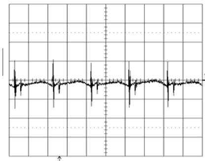
Output voltage ripple (20mV/div.) at: T_{ref} = +25^\circ\text{C} , I_O = 6\text{ A} resistive load, V_I = 12.0\text{ V} . Time scale: 2 \mu\text{s}/\text{div} . See the filter in the Output ripple and noise section (EMC Specification).
