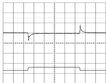
Output voltage response to load current step- change (3-6-3 A) at: T_{ref} = +25^\circ\text{C} , V_I = 12.0\text{ V} . Top trace: output voltage (100mV/div.). Bottom trace: load current (10 A/div.). Time scale: 0.1 ms/div.
