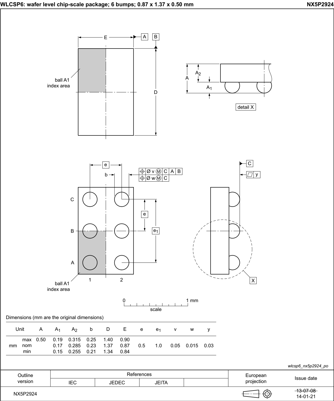
Fig 22. Package outline NX5P2924
