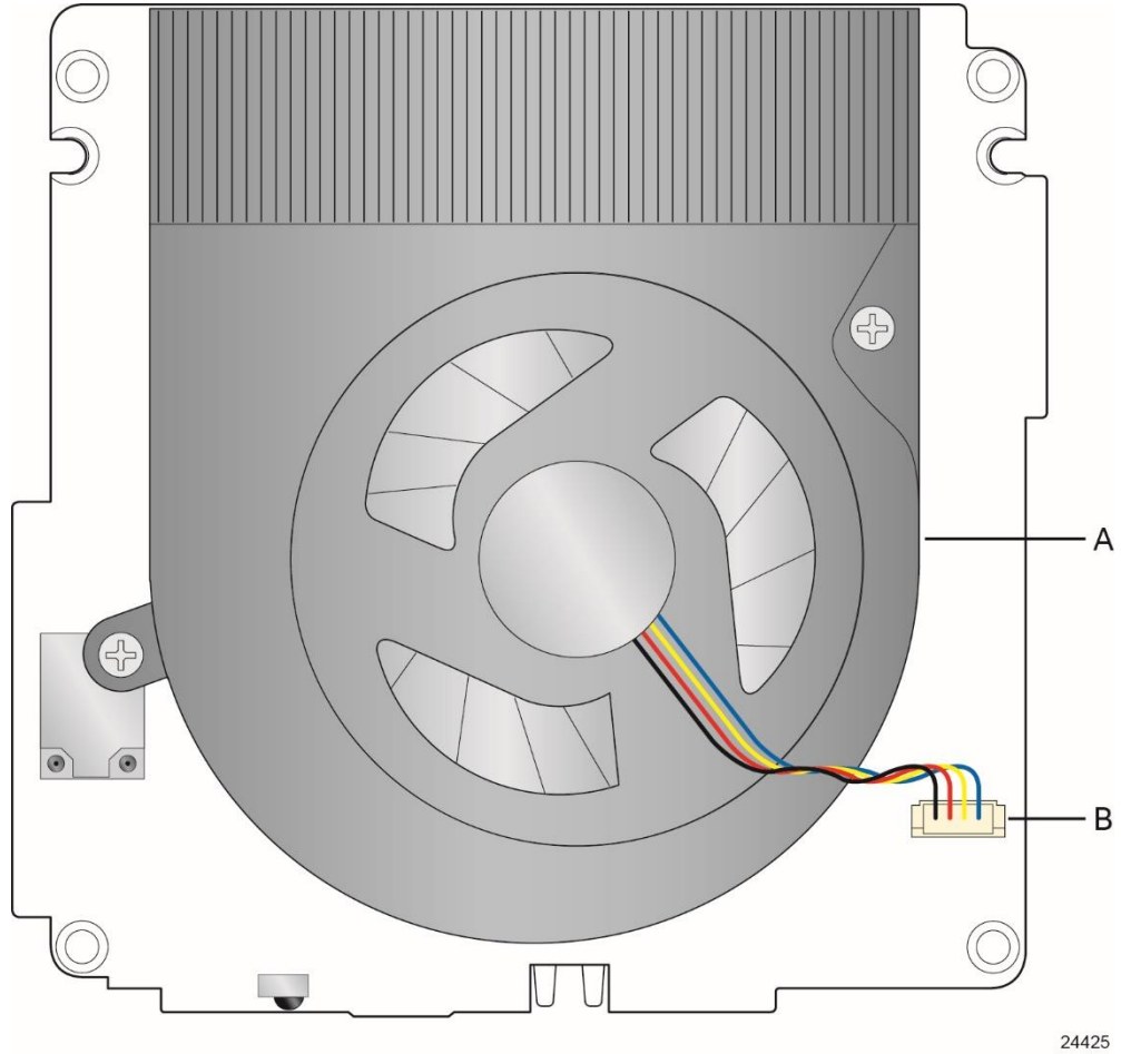
Figure 6. Thermal Solution and Fan Header
