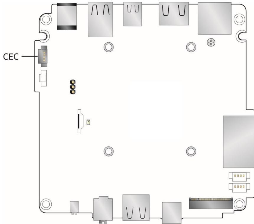
Figure 8. CEC Connector
