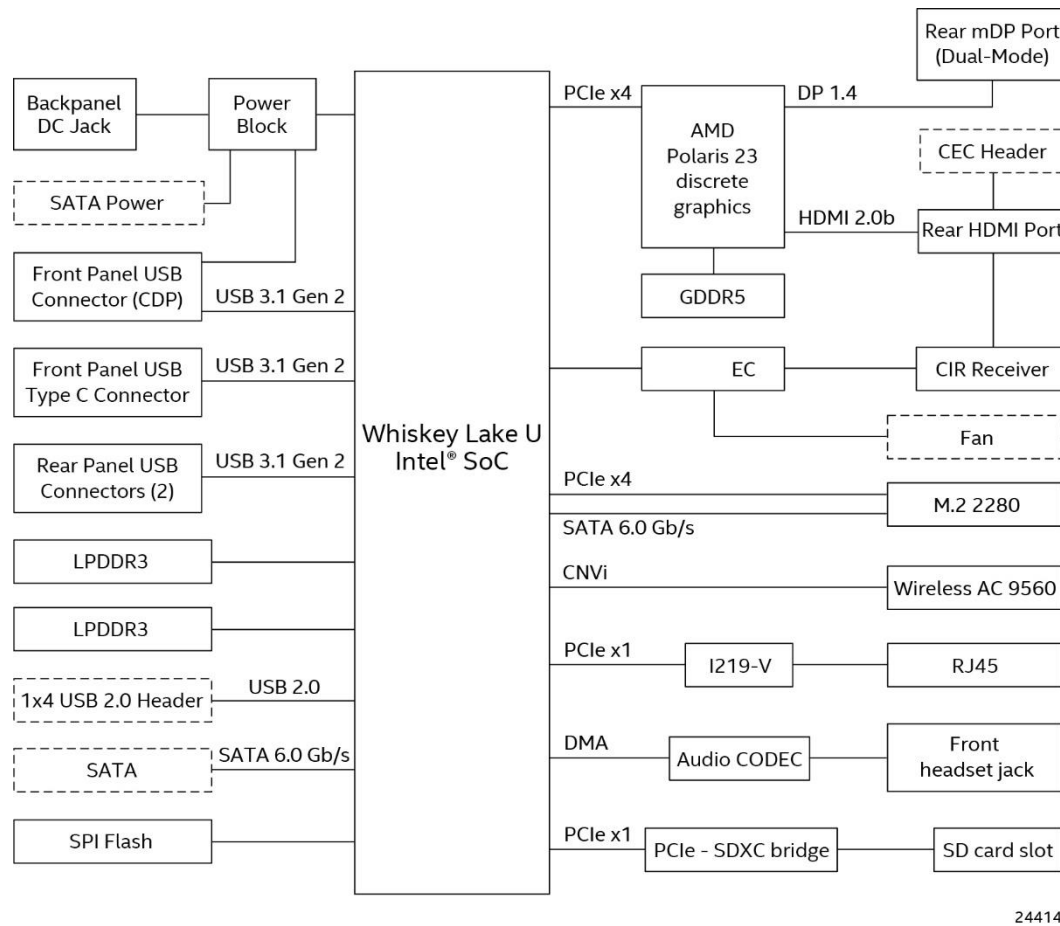
Figure 3. Block Diagram
