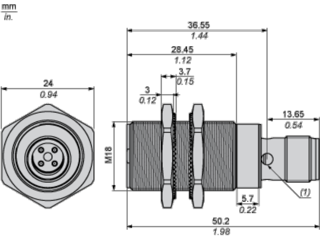
(1) LED
