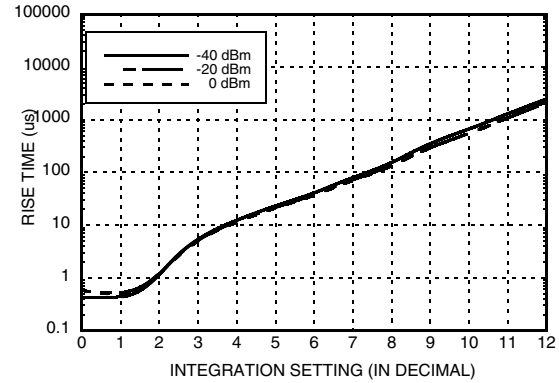
Rise Settling Time [3] vs. SCI Setting over Input Power
