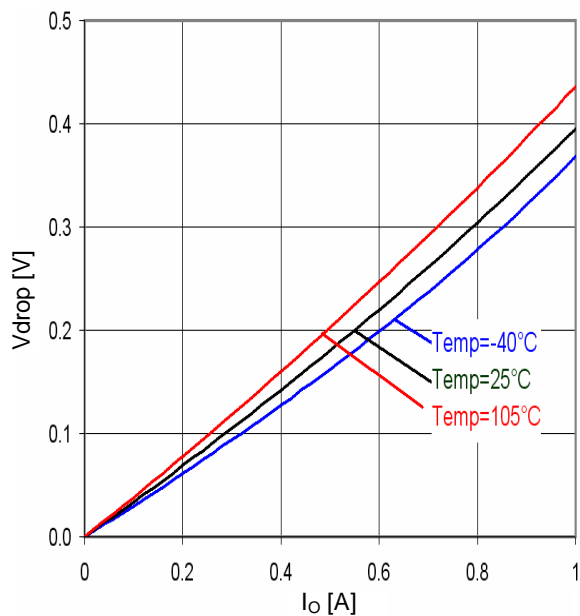
Fig.37 Minimum dropout Voltage 5 (V CC =5.5V, Ta=25°C)
