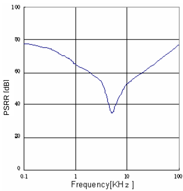
Fig.33 PSRR ( I_o =0mA)
