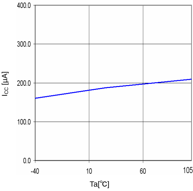
Fig.22 T_a - I_{cc}
