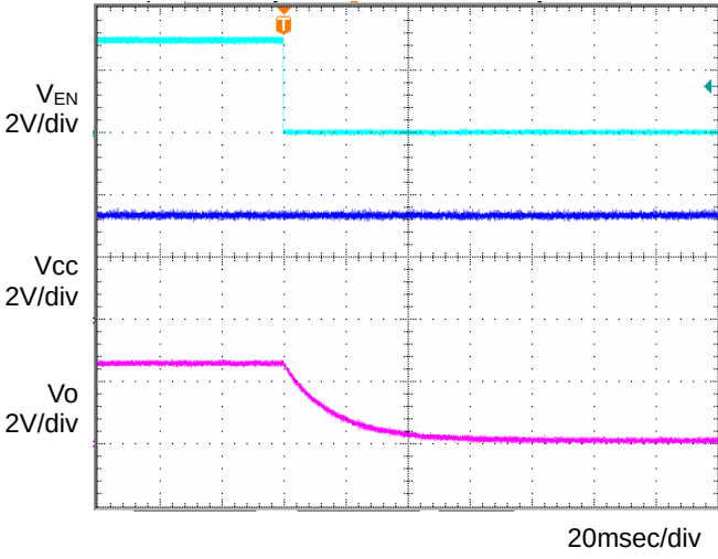
Fig.20 OFF sequence 2 Co=1μF,Ta=105°C
