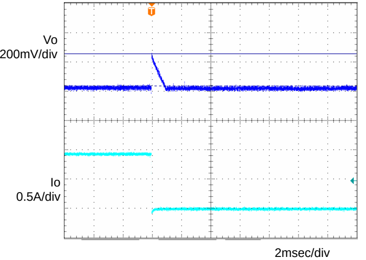
Fig.6 Transient Response (1.0→0A) Co=1µF, Ta=-40°C
