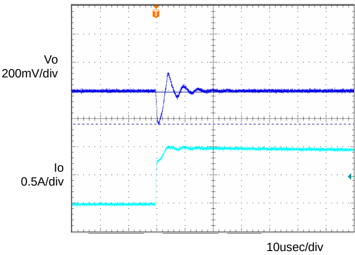
Fig.4 Transient Response (1.0→0A) Co=1µF, Ta=25°C
