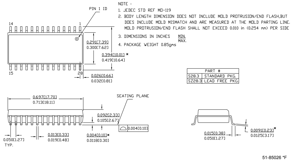
Figure 24. 28-pin (300-Mil) Molded SOIC
