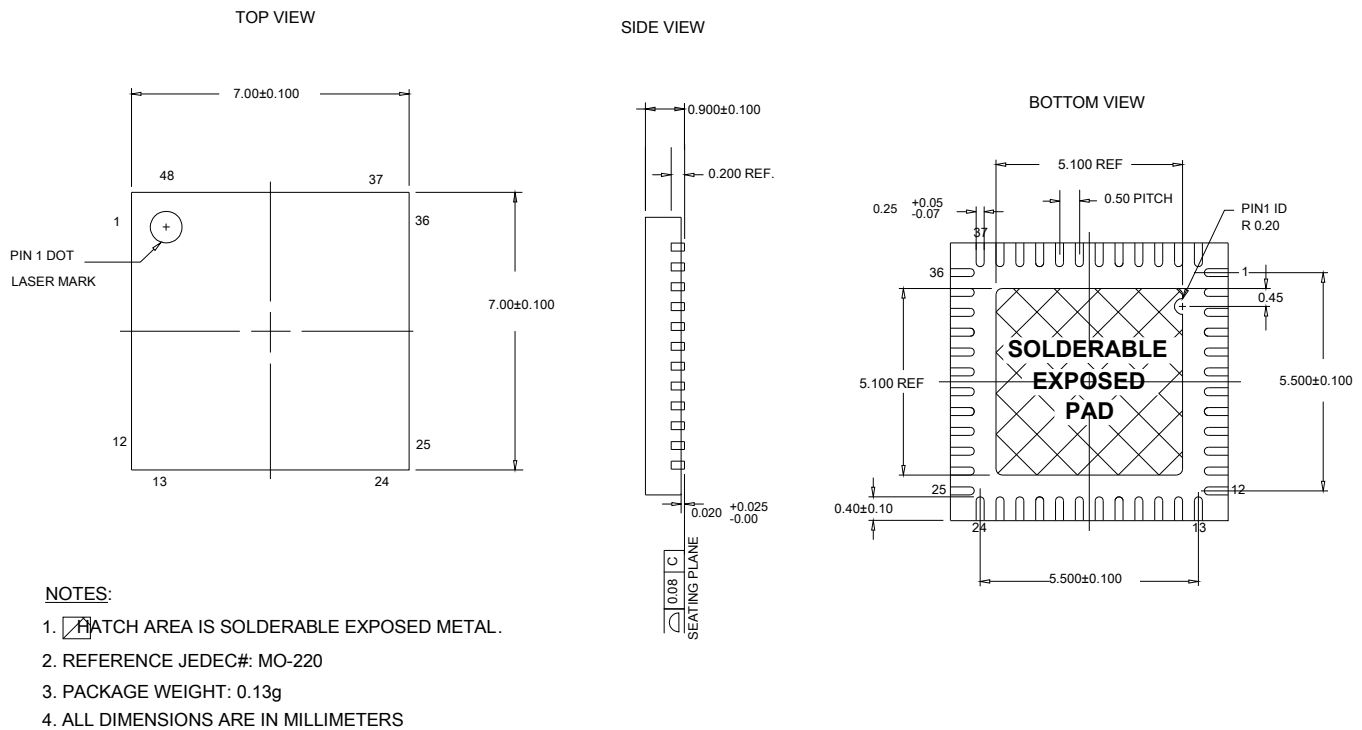
Figure 27. 48-pin QFN 7 × 7 × 0.90 mm (Sawn Type)
