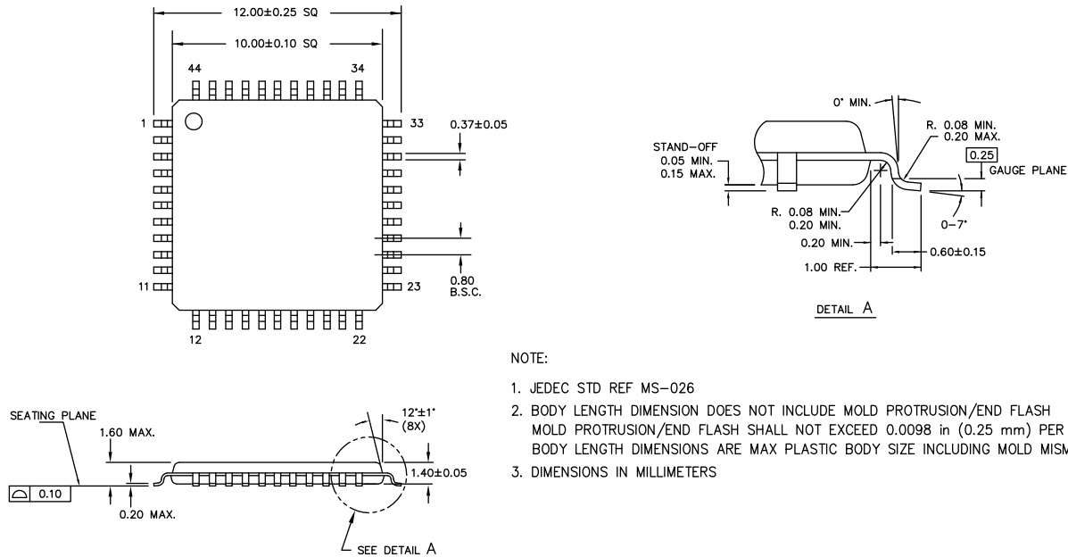
Figure 25. 44-pin TQFP
