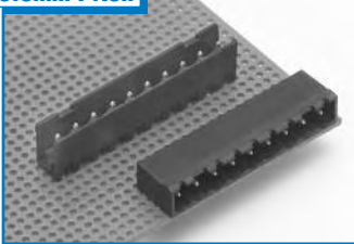
ELFH Closed Ends Hor/Ver ELFH Open Ends Hor/Ver . . Page 33 15A / 300V
