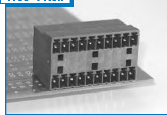
ELVA 2-Tier Aligned H/V . . . Page 23 12A / 300V
