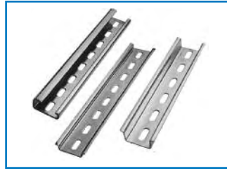
DIN Mounting Accessories . . . . . Page 134
