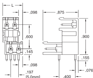
ELFD—Horizontal
