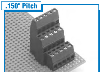
.150" Pitch
