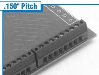
.150" Pitch
