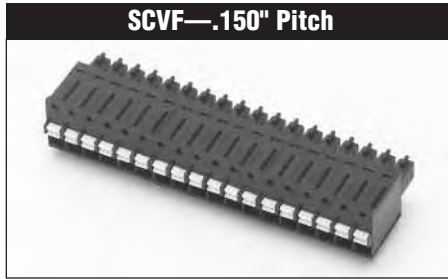
SCVF—.150" Pitch—Eared
