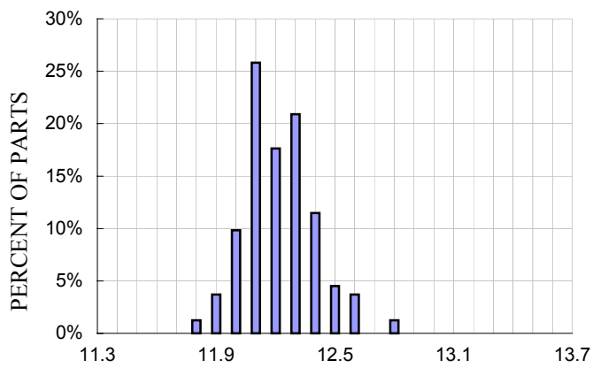
Y-axis Sensitivity Distribution at Yout, V_{DD}=3V
