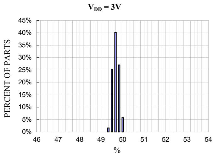
X-axis Zero g Bias Distribution at Xout, V DD =3V
