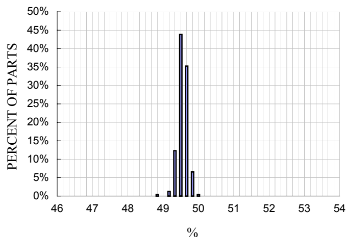
Y-axis Zero g Bias Distribution at Xout, V DD =3V
