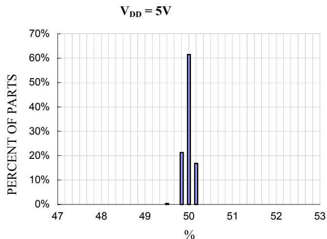
X-axis Zero g Bias Distribution at Xout, V DD =5V
