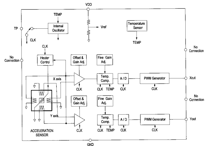
MXD7202GL/HL/ML/NL FUNCTIONAL BLOCK DIAGRAM
