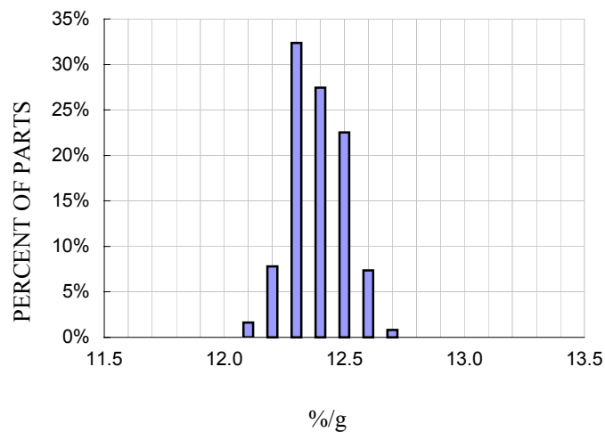
X-axis Sensitivity Distribution at Xout, V DD =5V
