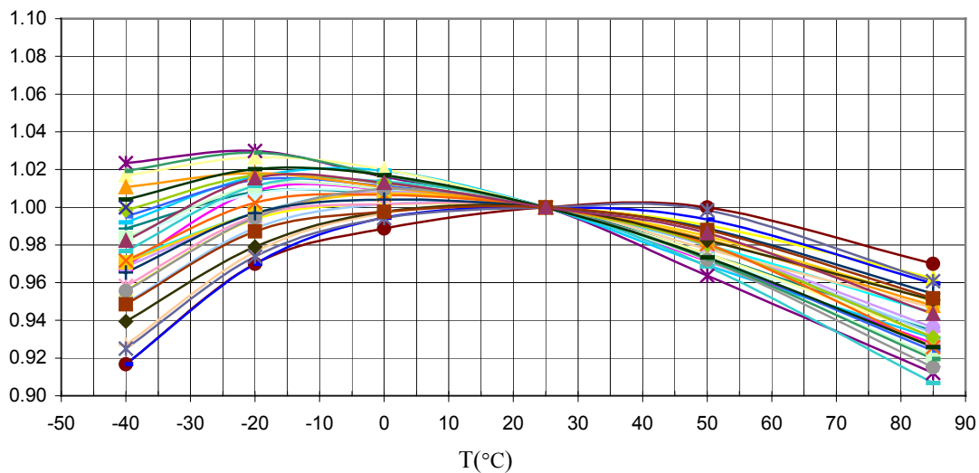
Normalized (with 25°C) Y-axis Sensitivity vs. Temperature, V_{DD}=5V
