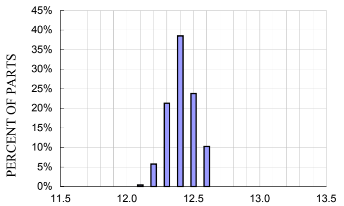
Y-axis Sensitivity Distribution at Yout, V_{DD}=5V
