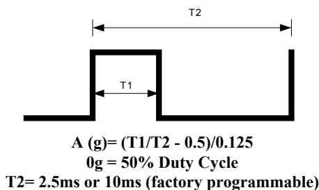
Figure 3: Typical output Duty Cycle
