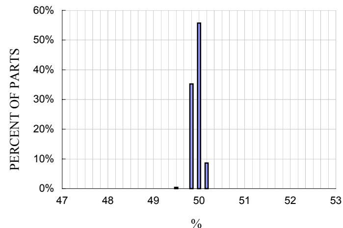
Y-axis Zero g Bias Distribution at Xout, V DD =5V
