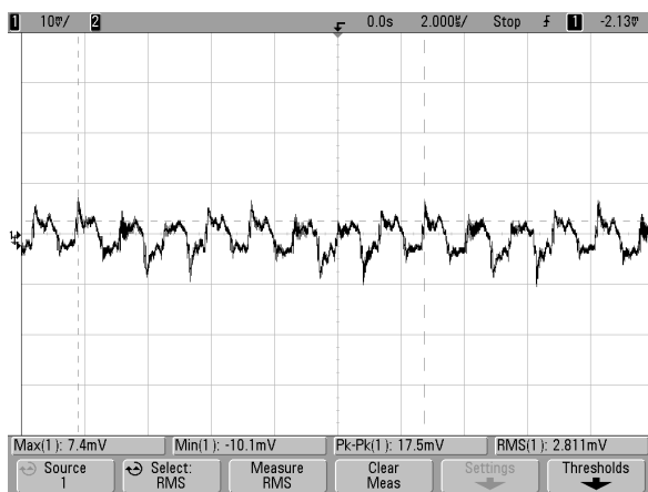
Output Voltage Ripple @ BW=20MHz Vin=48V, Iout=0A, Cout=700µF, Ta=+25°C, 2µS/div
