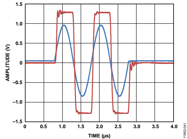
Figure 19. Overdrive Recovery
