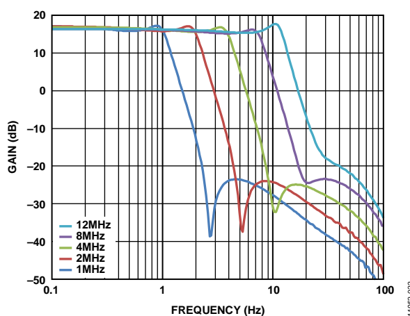
Figure 14. Filter Response
