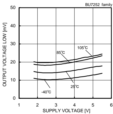
Fig. 29 Output Voltage Low - Supply Voltage( R_L=10[k\Omega] )
