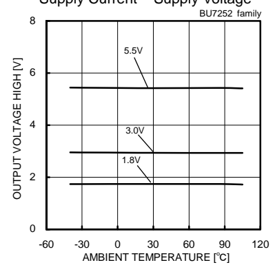
Fig. 28 Output Voltage High - Ambient Temperature ( R_L=10[k\Omega] )
