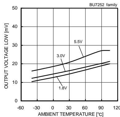
Fig. 30 Output Voltage Low - Ambient Temperature( R_L=10[k\Omega] )
