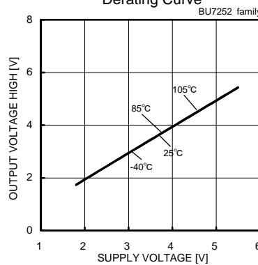
Fig. 27 Output Voltage High - Supply Voltage ( R_L=10[k\Omega] )
