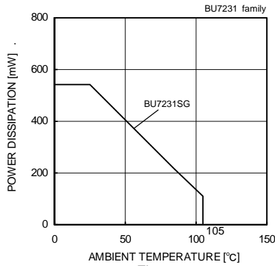
Fig. 46 Derating Curve
