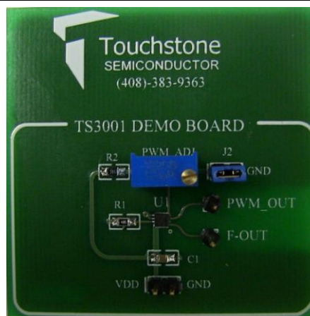
Figure 2. TS3001 Evaluation Board
