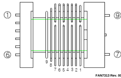
Figure 5. Transformer Schematic
