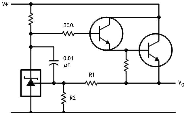
Series Regulator
