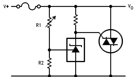
Crow Bar
