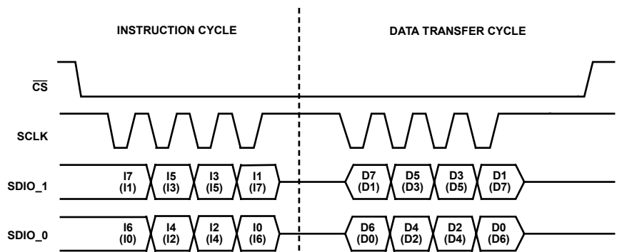
Figure 55. 2-Bit Mode Read Timing—Clock Stall High
