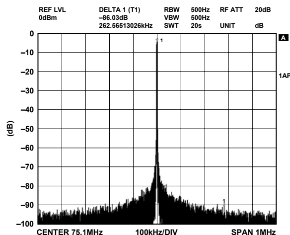
Figure 17. f_{OUT} = 75.1 MHz, f_{CLK} = 500 MSPS, NBSFDR, \pm 1 MHz
