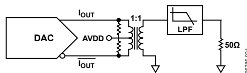
Figure 35. Typical DAC Output Termination Configuration
