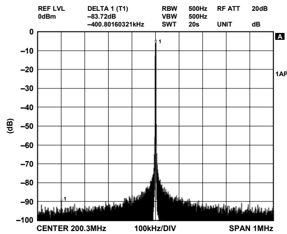
Figure 18. f_{OUT} = 200.3 MHz, f_{CLK} = 500 MSPS, NBSFDR, \pm 1 MHz
