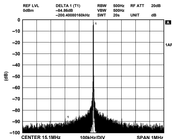
Figure 16. f_{OUT} = 15.1 MHz, f_{CLK} = 500 MSPS, NBSFDR, \pm 1 MHz
