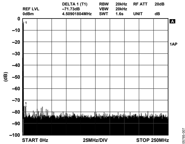
Figure 7. f_{OUT} = 1.1 MHz, f_{CLK} = 500 MSPS, Wideband SFDR
