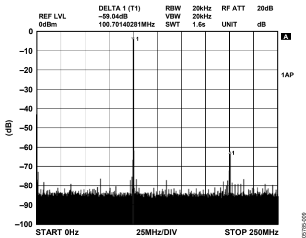
Figure 9. f_{OUT} = 100.3 MHz, f_{CLK} = 500 MSPS, Wideband SFDR
