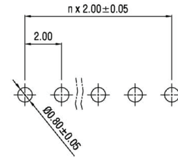
PCB Layouts
