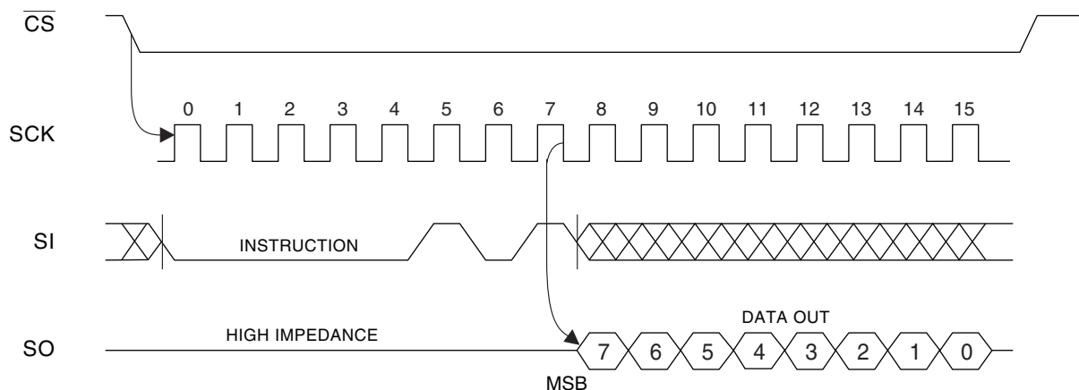
Figure 4-4. RDSR Timing
