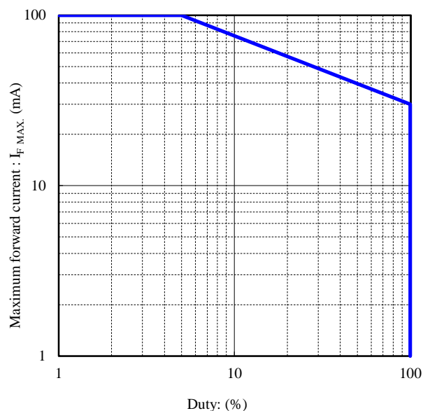
Duty cycle vs. Maximum forward current
