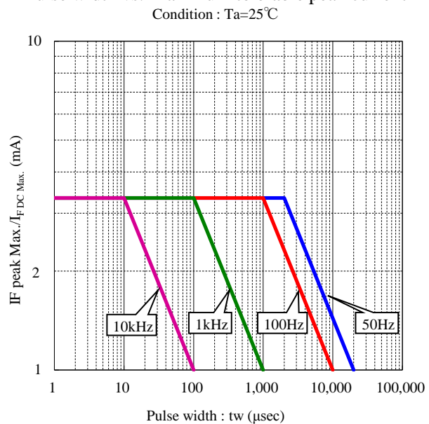
Pulse width vs. Maximum tolerable peak current
