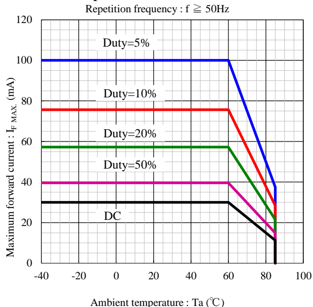
Ambient temp. vs. Maximum forward current
