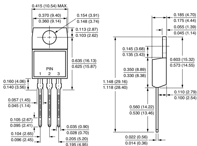
TO-220AB
