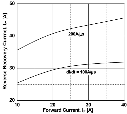
Figure 19. Reverse Current
