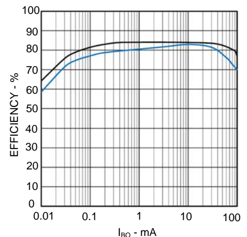
Efficiency vs Output Load Current
