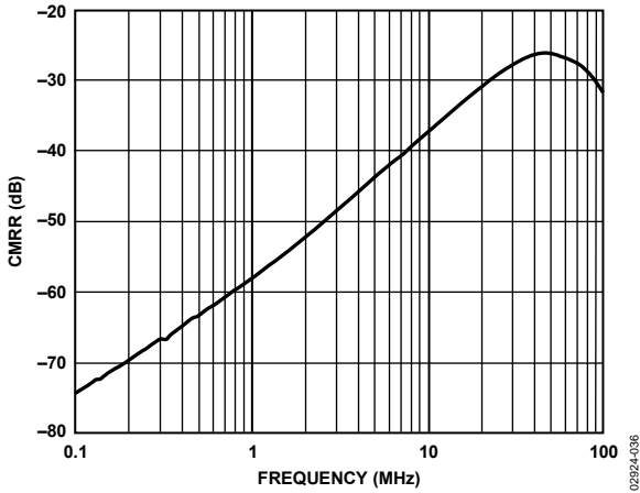
Figure 36. CMRR vs. Frequency (See Figure 50)
