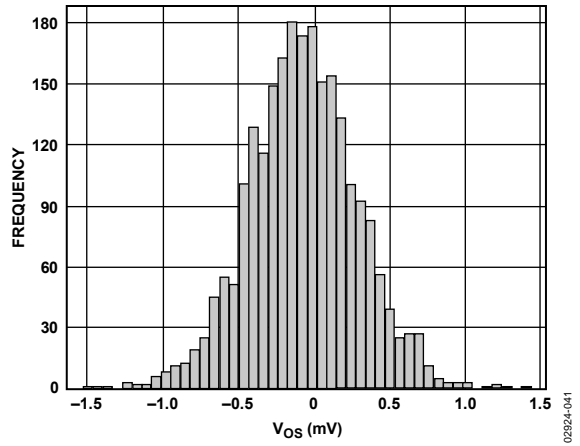
Figure 41. Initial Offset
