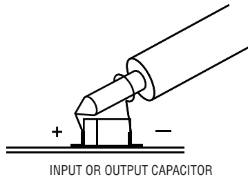
Figure 2. Measuring V_{IN} or V_{OUT} Ripple
