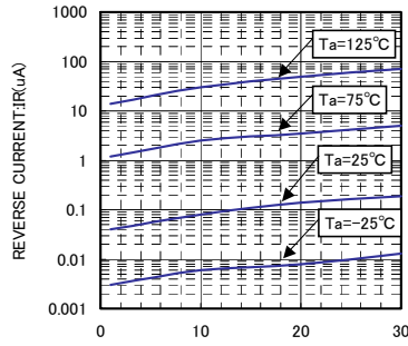
VR-IR CHARACTERISTICS
