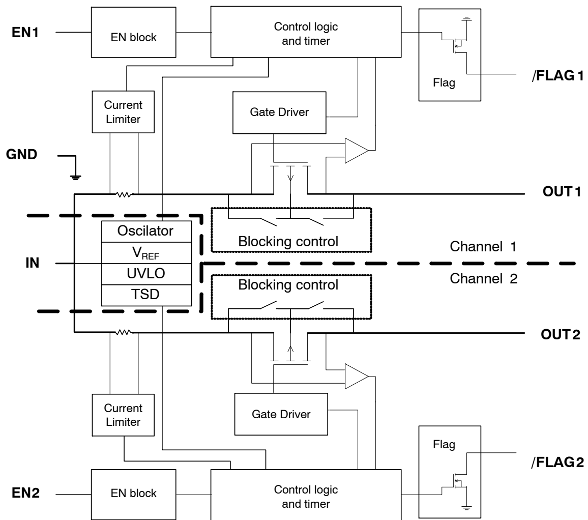
Figure 5. Block Diagram
