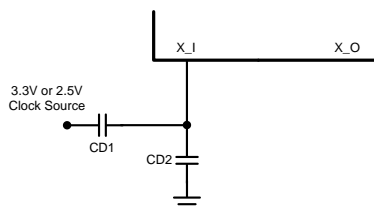
Figure 24. Clock Divider
