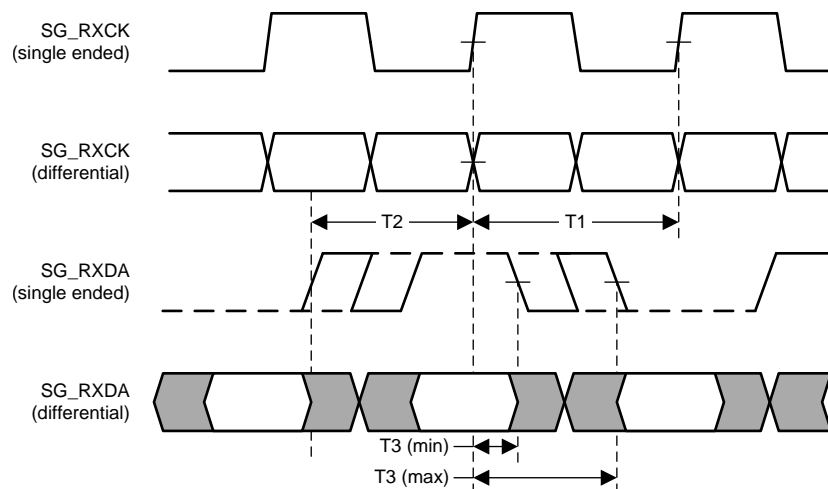
Figure 4. SGMII Timing
