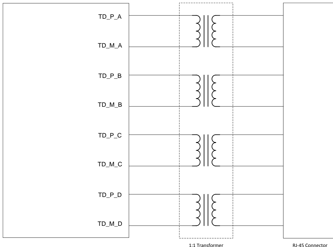
Figure 23. Magnetics Connections
