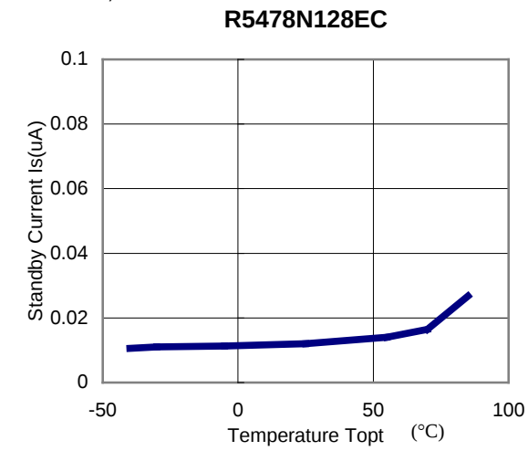
20) Standby Current vs. Temperature Vdd=3.9V, V-=0V
