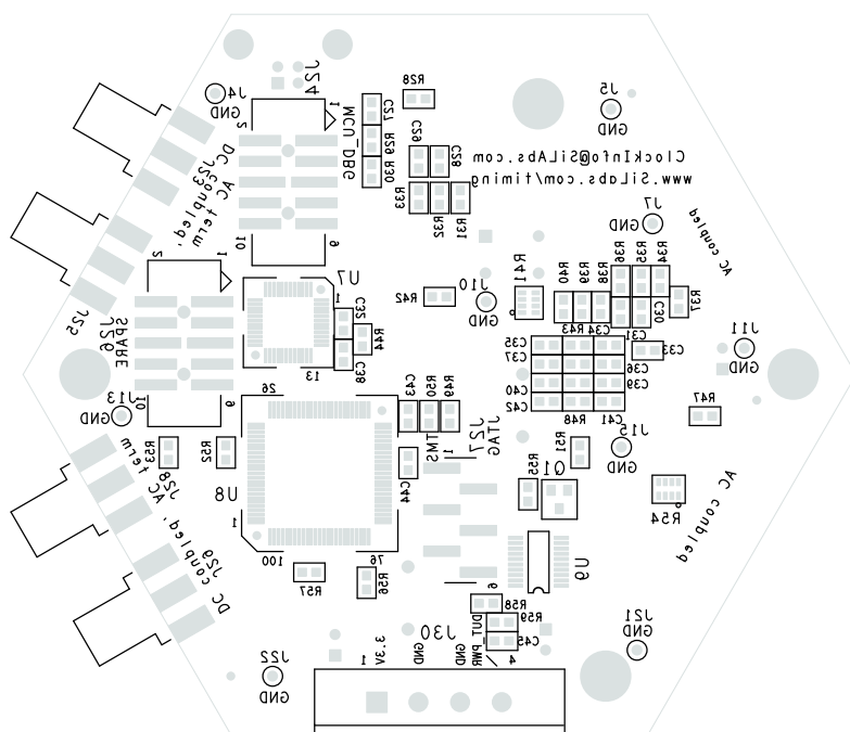
Figure 18. Silkscreen Bottom
