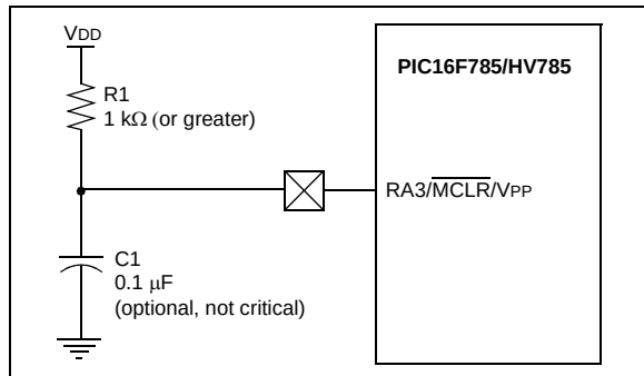
FIGURE 15-2: RECOMMENDED \overline{MCLR} CIRCUIT
