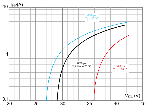
Figure 5. Peak pulse current versus clamping voltage (typical values) ESDCAN03
