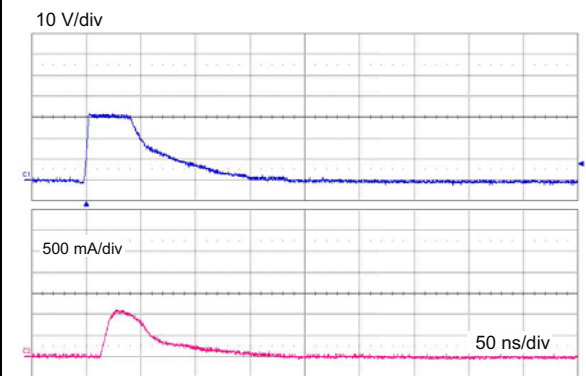
Figure 9. Response to ISO 7637-3 Pulse 3b ( U_s = +100\text{ V} )
