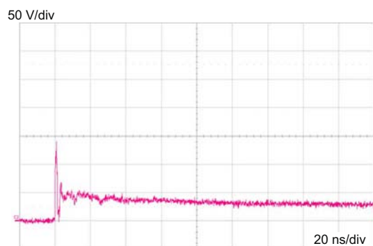
Figure 6. ESD response to ISO 10605 - C = 150 pF, R = 330 \Omega (+8 kV contact)
