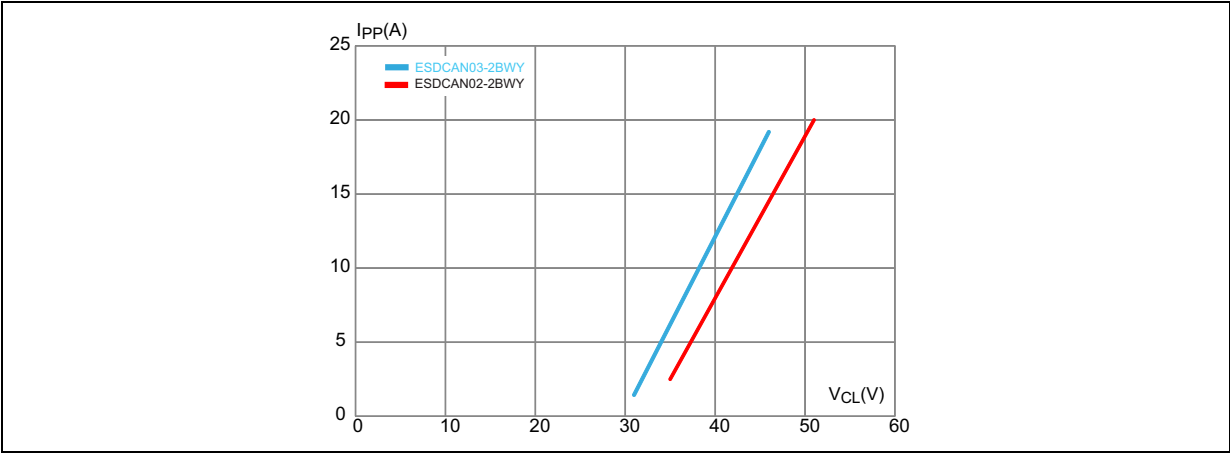
Figure 10. TLP measurements
