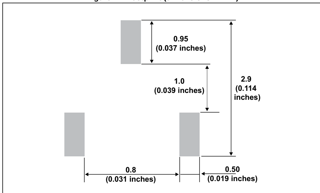
Figure 12. Footprint (dimensions in mm)
