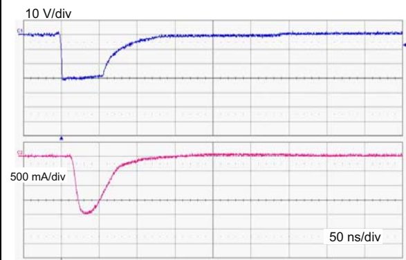
Figure 8. Response to ISO 7637-3 Pulse 3a ( U_s = -150\text{ V} )
