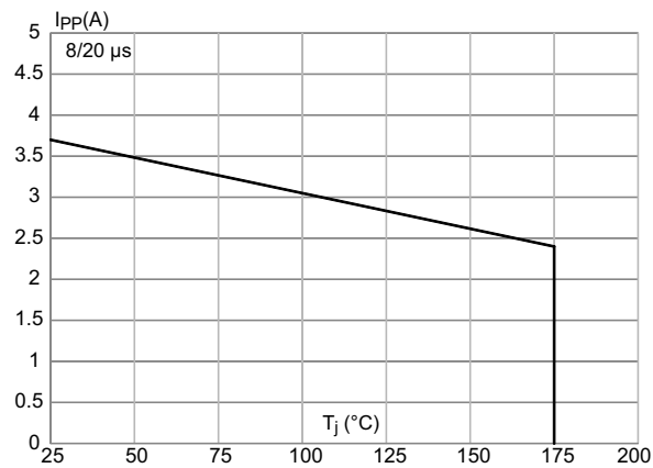
Figure 2. Peak pulse current versus initial junction temperature (maximum values)
