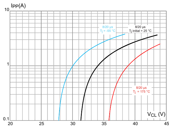
Figure 4. Peak pulse current versus clamping voltage (typical values) ESDCAN02
