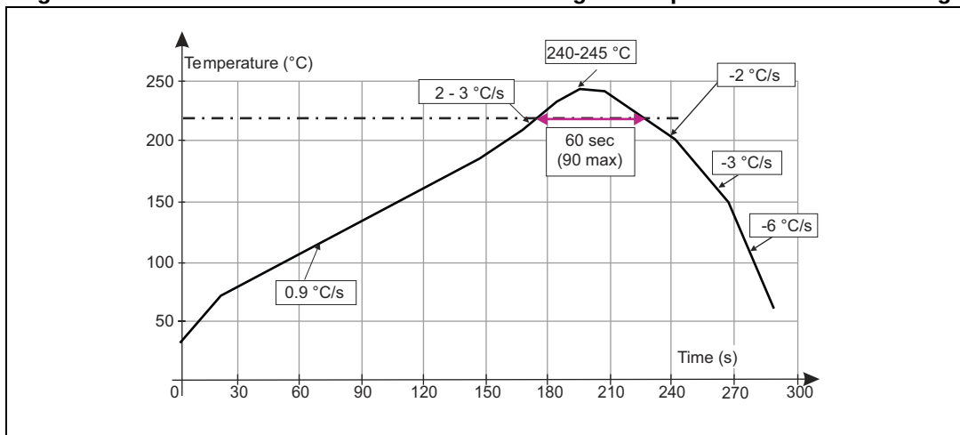
Figure 13. ST ECOPACK® recommended soldering reflow profile for PCB mounting
