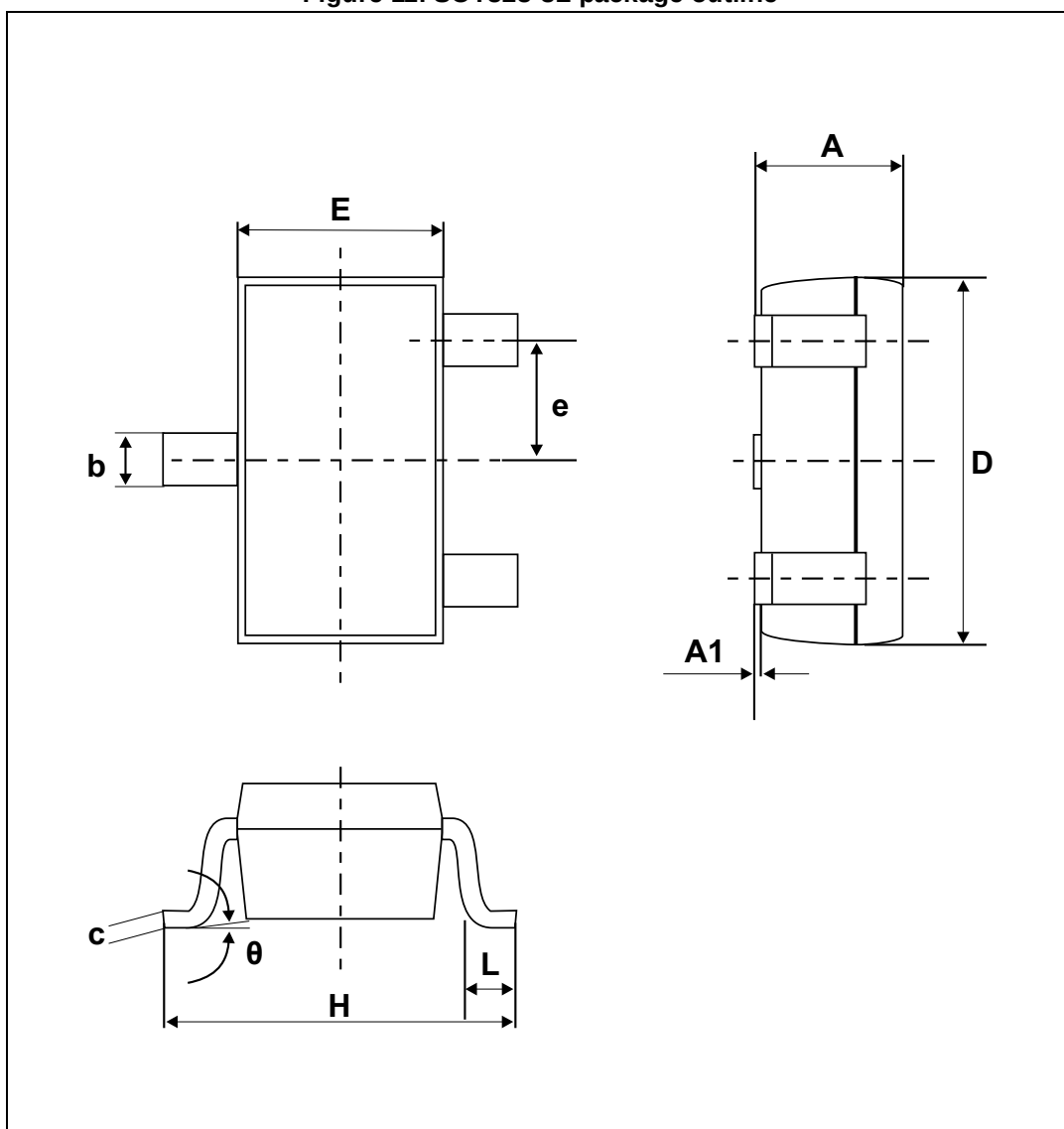
Figure 11. SOT323-3L package outline
