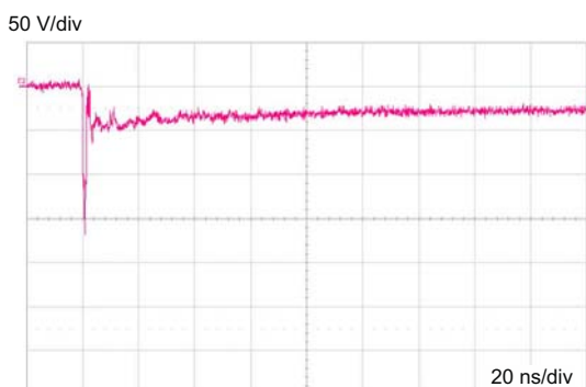
Figure 7. ESD response to ISO 10605 - C = 150 pF, R = 330 \Omega (-8 kV contact)
