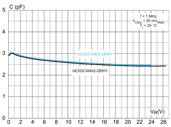
Figure 3. Junction capacitance versus reverse voltage applied (typical values)
