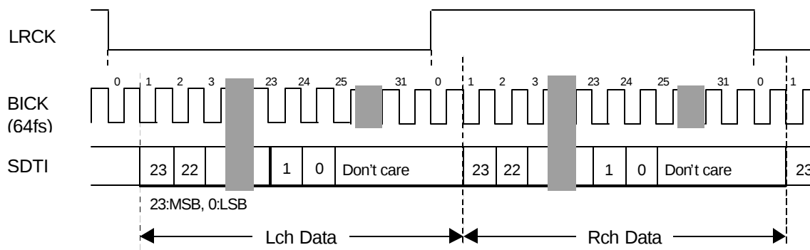
Figure 4. Mode 3 Timing
