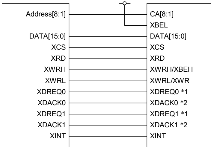
16-bit CPU (XWRH/XWRL) connection example
