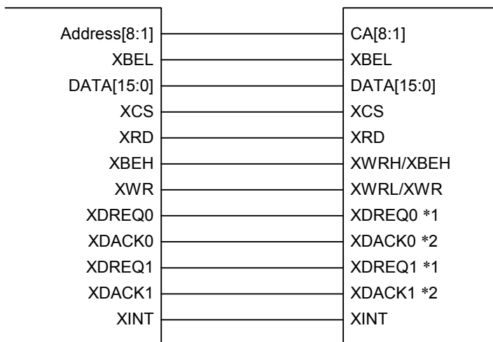
16-bit CPU (XBEH/XBEL) connection example
