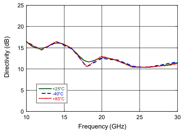
Directivity
