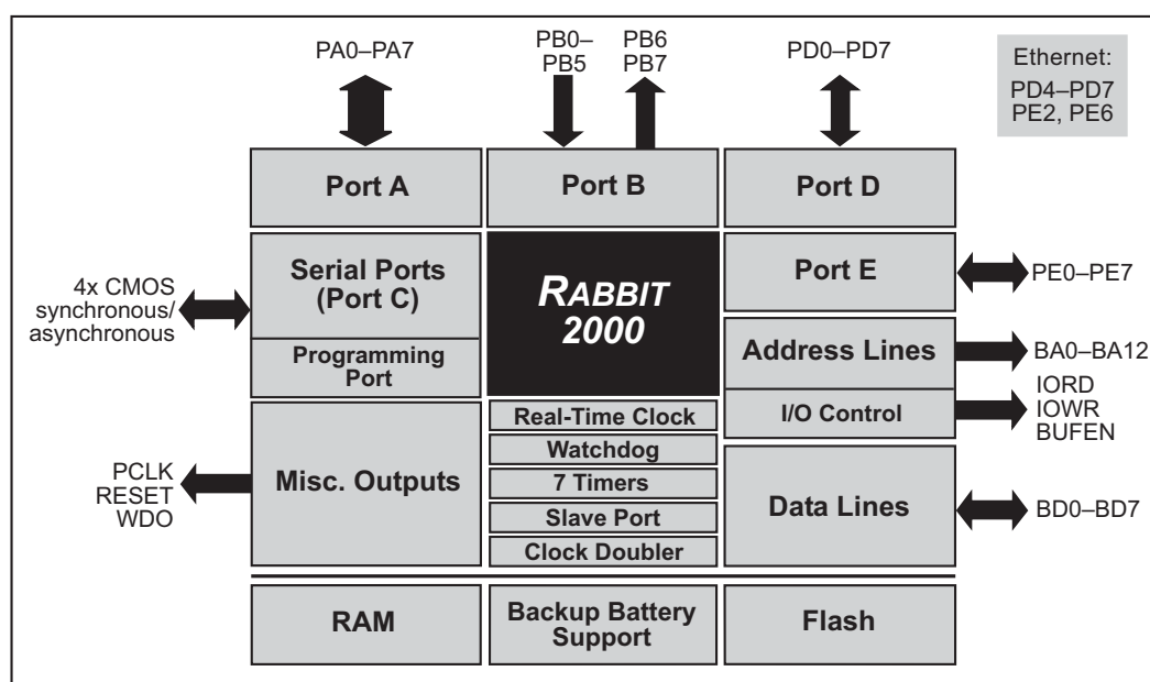
Figure 5. Rabbit Subsystems
