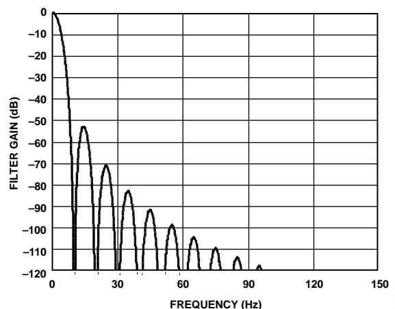
Figure 33. Sinc 4 Filter Response (FS[9:0] = 480)
