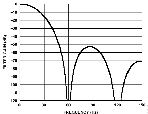
Figure 32. Sinc 4 Filter Response (FS[9:0] = 80)
