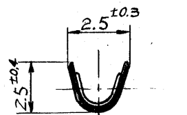
SECT. "A"- "A"
