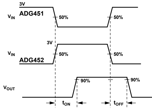
Figure 19. Switching Times
